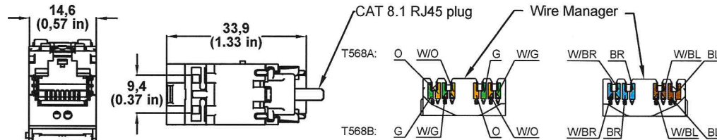
EIGHT CONTACT RJ45 PLUG FOR CONDUCTORS WITH AN INSULATION O.D. RANGE 0.039 - 0.063 AND JACKET O.D. RANGE 0.236 - 0.393
