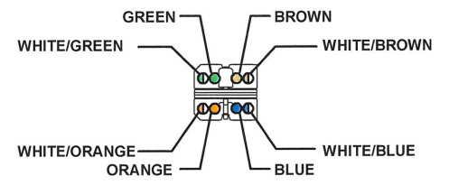
T568A Pin Assignment
