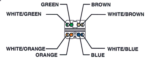
T568A Pin Assignment
